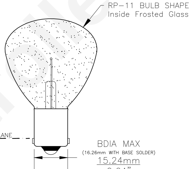
90° VIEW
